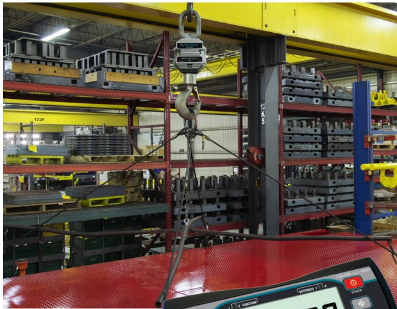
Coupling an MSI-8000 remote display and MSI-6360 crane scale is a simple and versatile wireless solution. Remotely view and operate the MSI-6360 as a seamless answer for most industrial applications.
